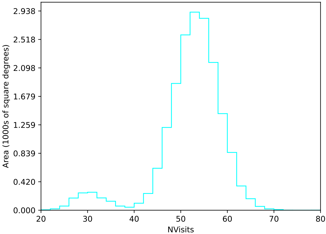
early_ss_template_fpextra2.0_v3.4_10yrs WFD u band: NVisits
