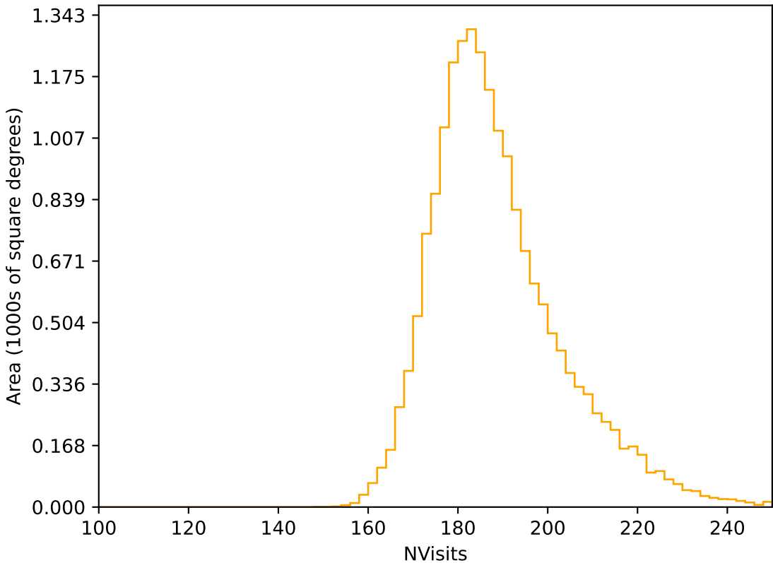
early_ss_template_fpextra2.0_v3.4_10yrs WFD r band: NVisits
