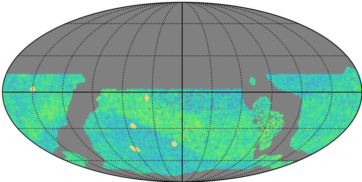
early_ss_template_fpextra2.0_v3.4_10yrs WFD i band: NVisits
