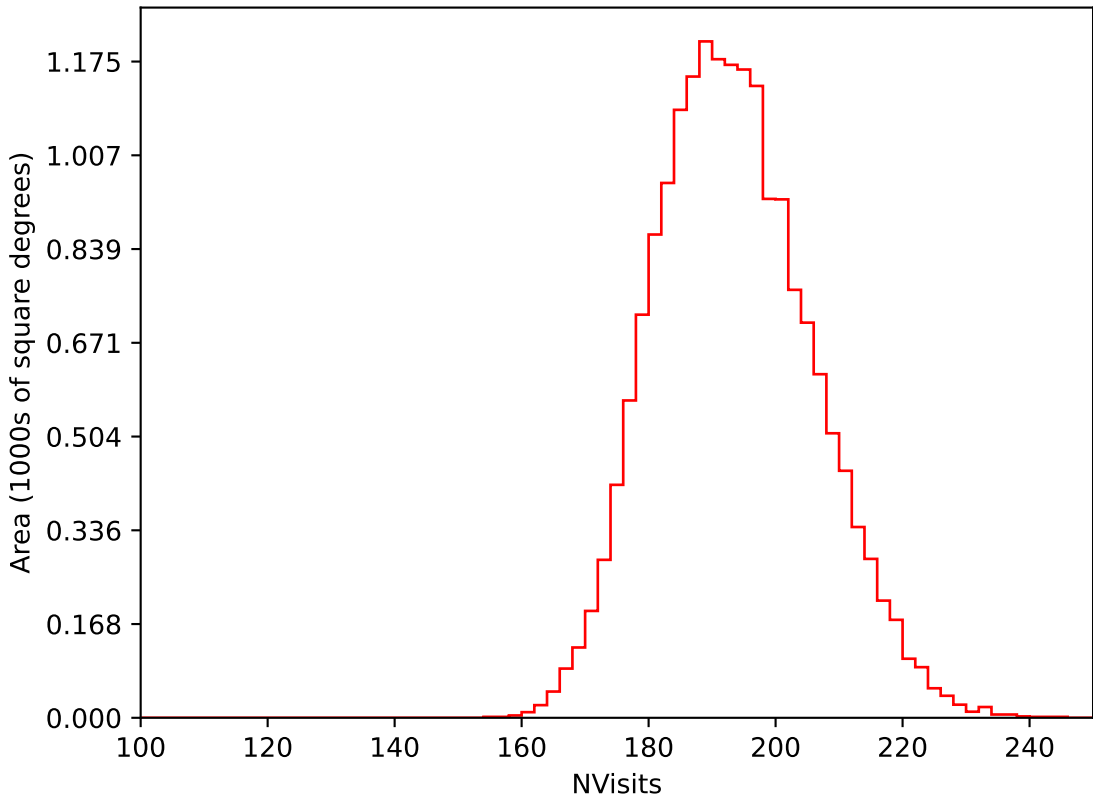
early_ss_template_fpextra2.0_v3.4_10yrs WFD i band: NVisits
