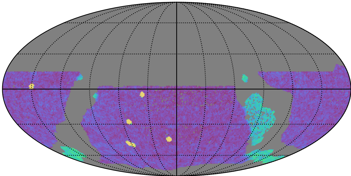
early_ss_template_fpextra2.0_v3.4_10yrs WFD g band: NVisits
