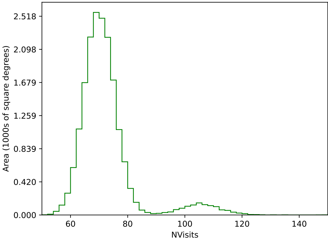
early_ss_template_fpextra2.0_v3.4_10yrs WFD g band: NVisits
