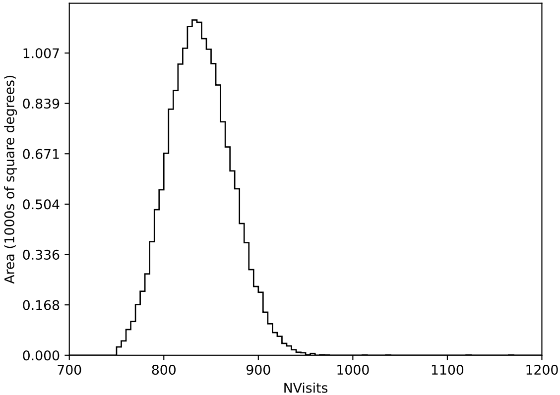
early_ss_template_fpextra2.0_v3.4_10yrs WFD all bands: NVisits
