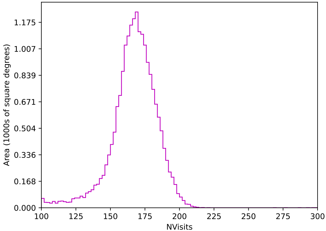
early_ss_template_fpextra2.0_v3.4_10yrs All sky z band: NVisits
