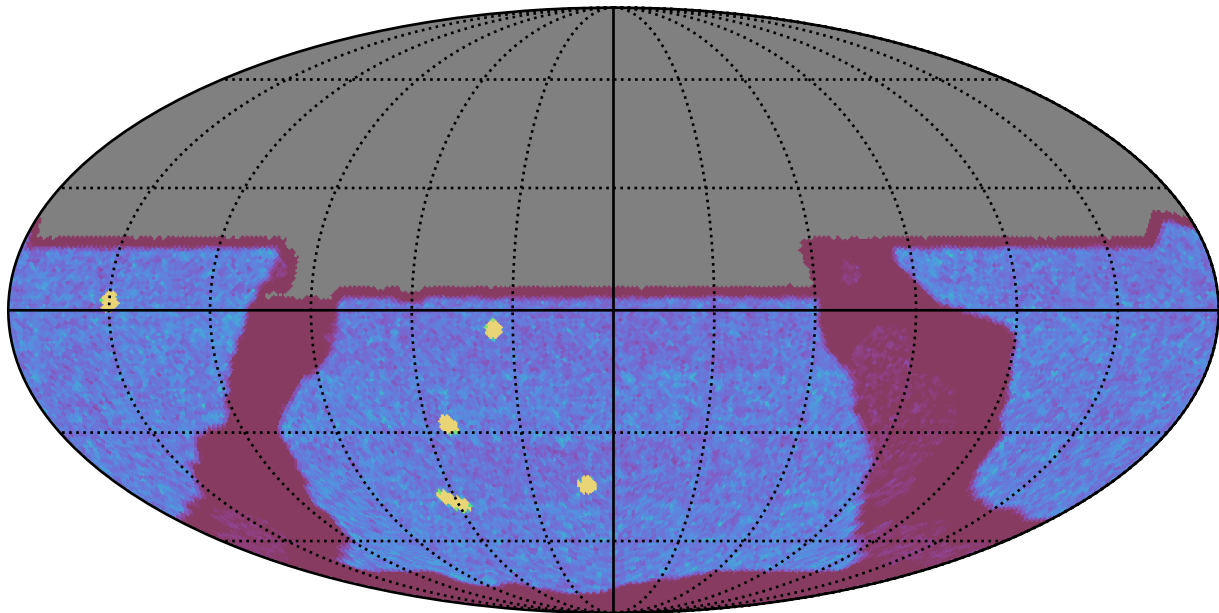
early_ss_template_fpextra2.0_v3.4_10yrs All sky y band: NVisits
