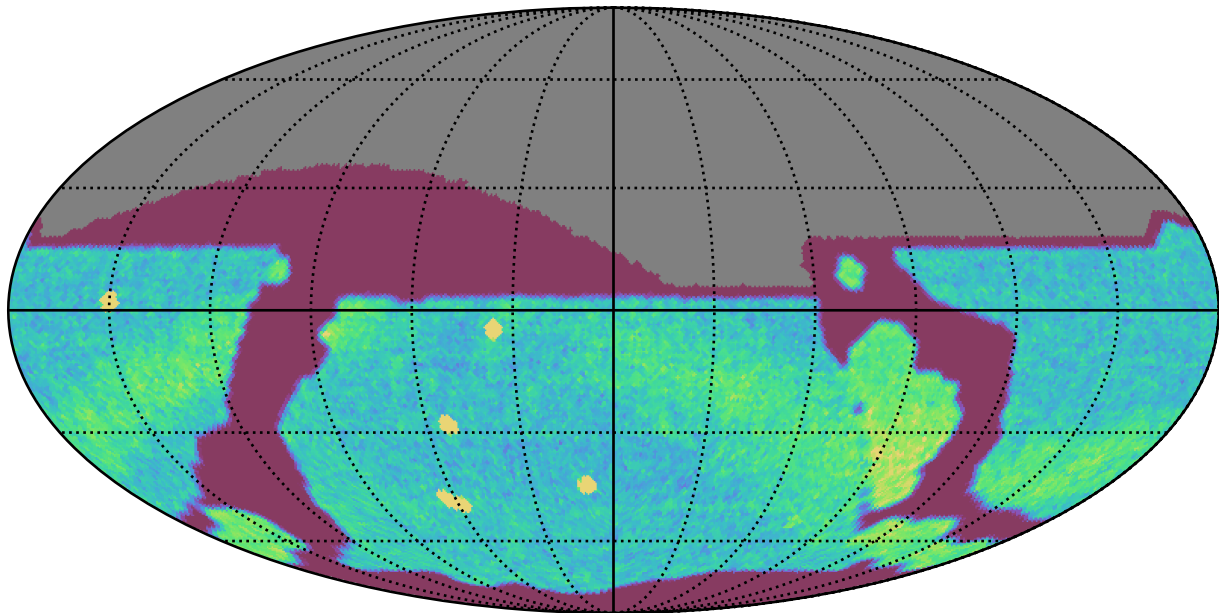
early_ss_template_fpextra2.0_v3.4_10yrs All sky r band: NVisits
