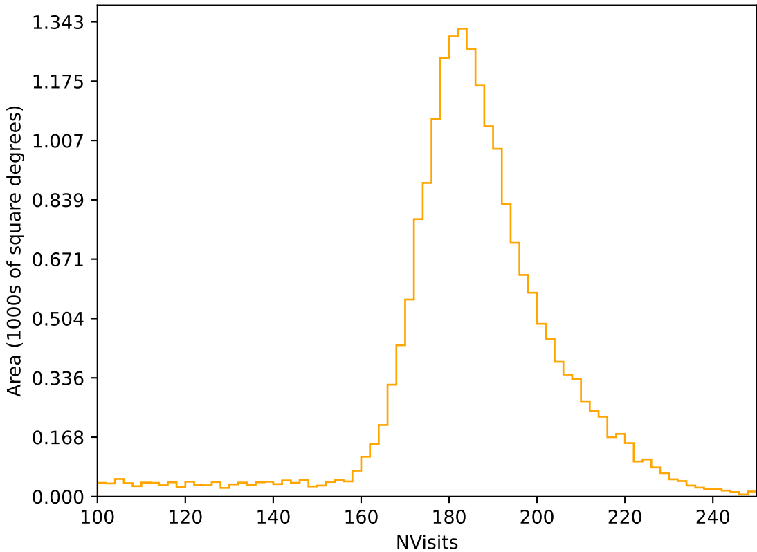
early_ss_template_fpextra2.0_v3.4_10yrs All sky r band: NVisits
