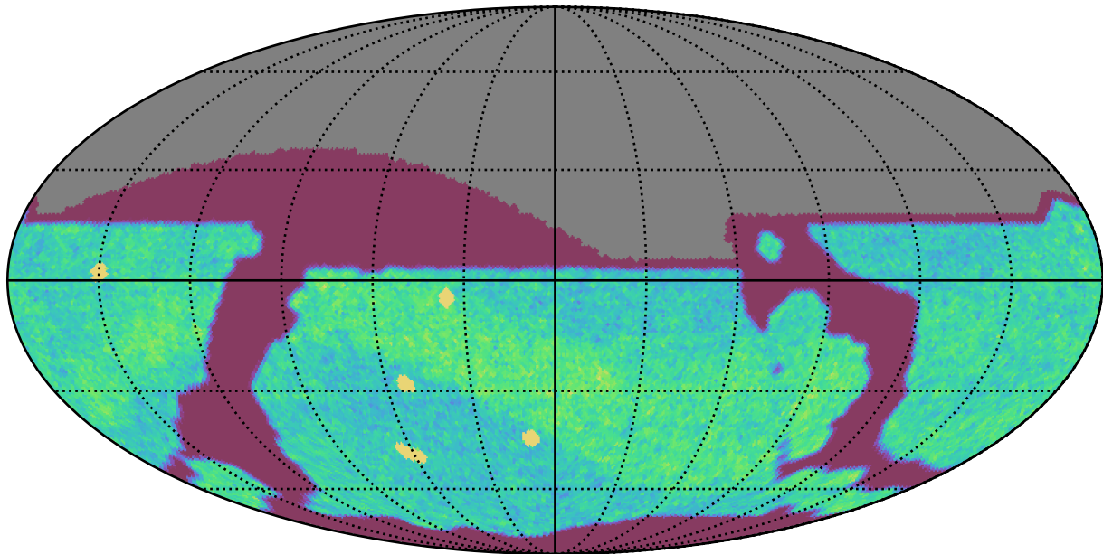
early_ss_template_fpextra2.0_v3.4_10yrs All sky i band: NVisits
