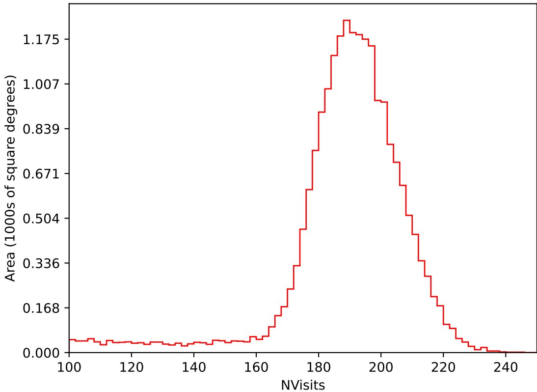
early_ss_template_fpextra2.0_v3.4_10yrs All sky i band: NVisits
