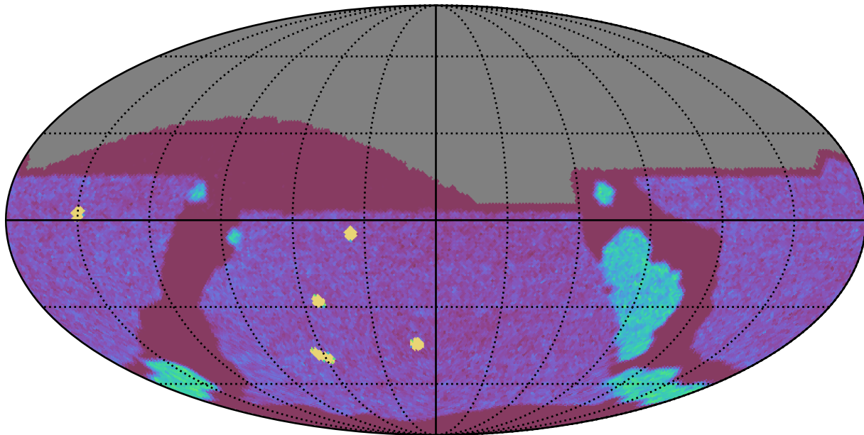
early_ss_template_fpextra2.0_v3.4_10yrs All sky g band: NVisits
