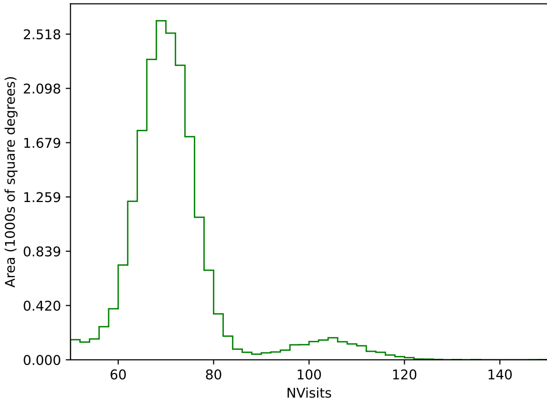
early_ss_template_fpextra2.0_v3.4_10yrs All sky g band: NVisits
