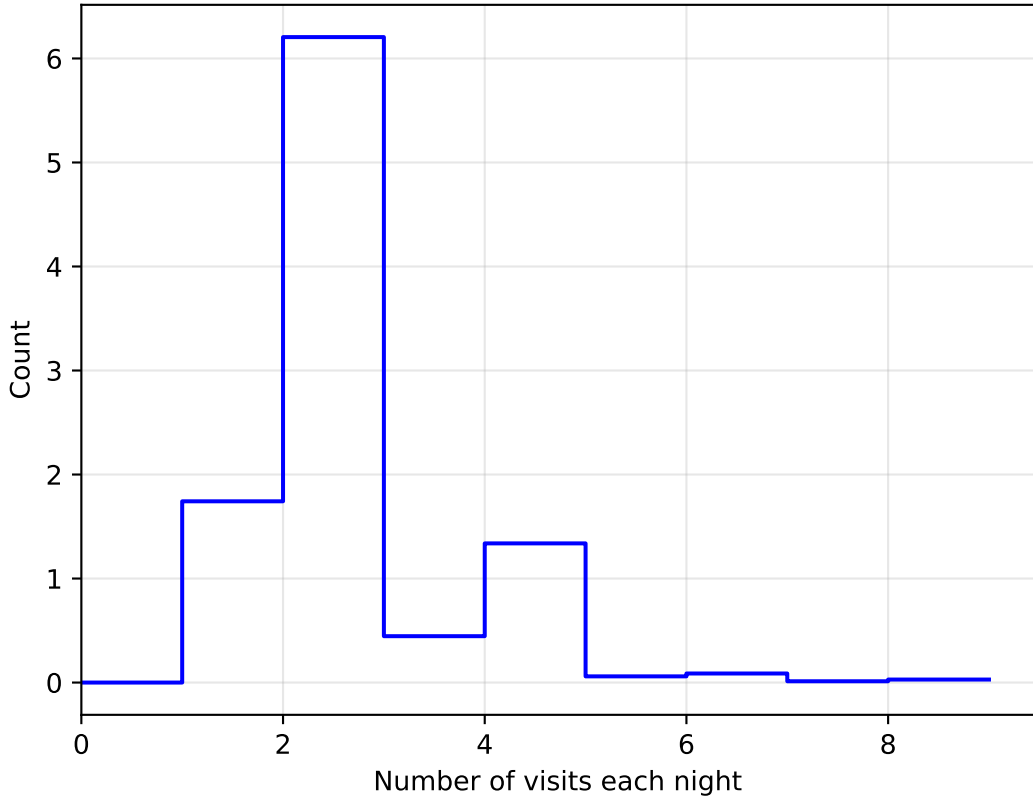
early_ss_template_fpextra2.0_v3.4_10yrs All sky: NVisitsPerNight 1e6
