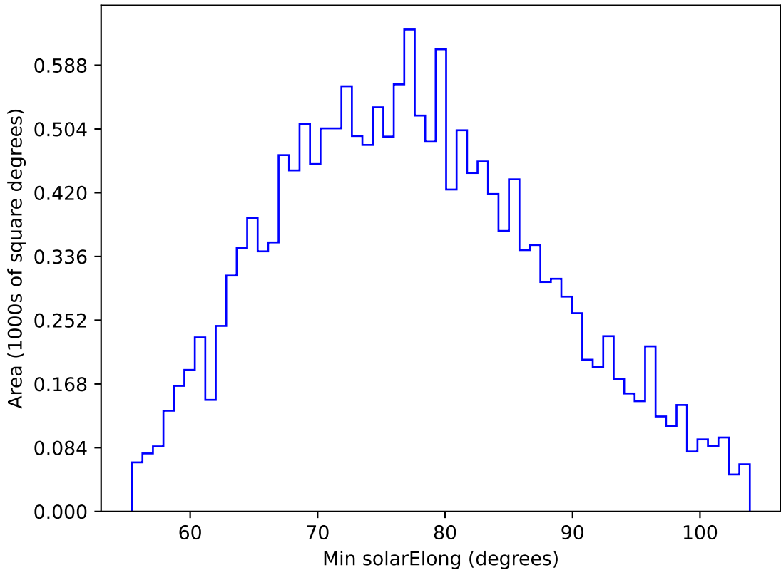
early_ss_template_fpextra2.0_v3.4_10yrs WFD u band: Min solarElong
