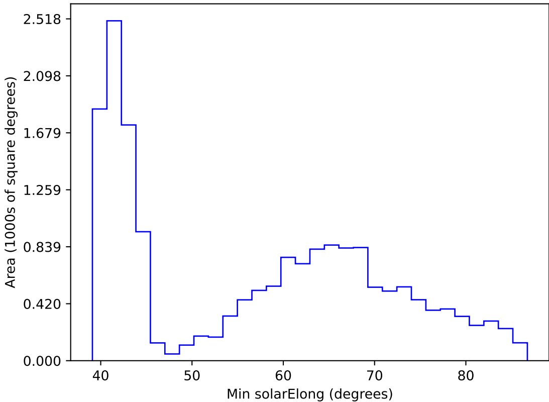
early_ss_template_fpextra2.0_v3.4_10yrs WFD r band: Min solarElong
