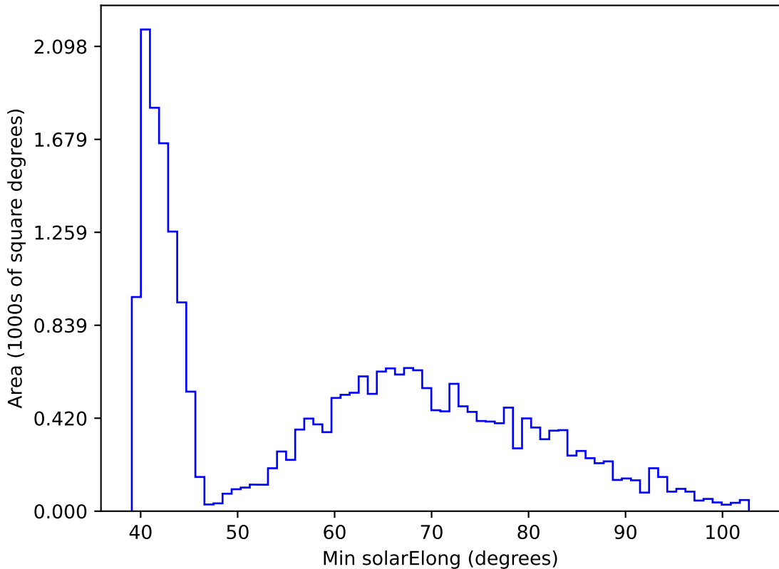
early_ss_template_fpextra2.0_v3.4_10yrs All sky r band: Min solarElong
