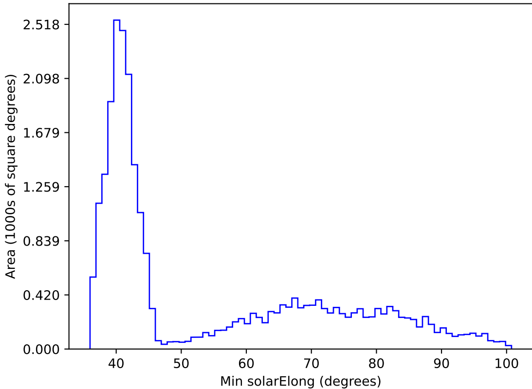
early_ss_template_fpextra2.0_v3.4_10yrs All sky i band: Min solarElong
