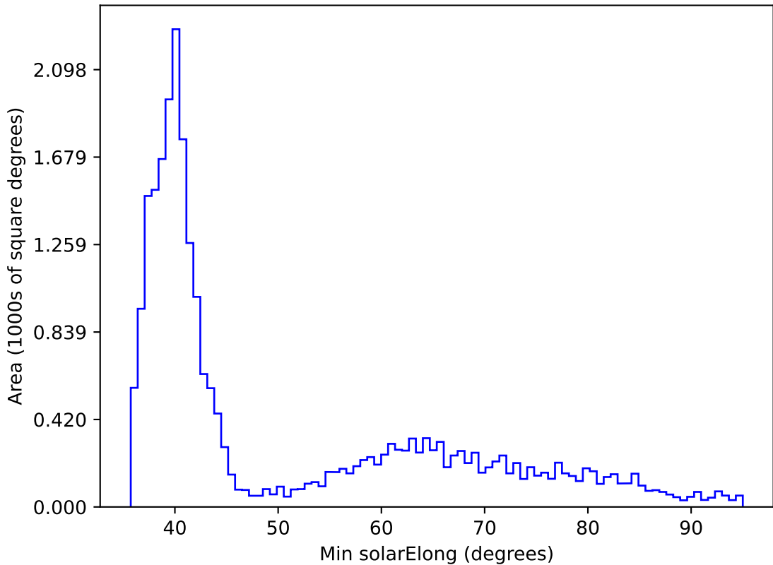
early_ss_template_fpextra2.0_v3.4_10yrs All sky all bands: Min solarElong
