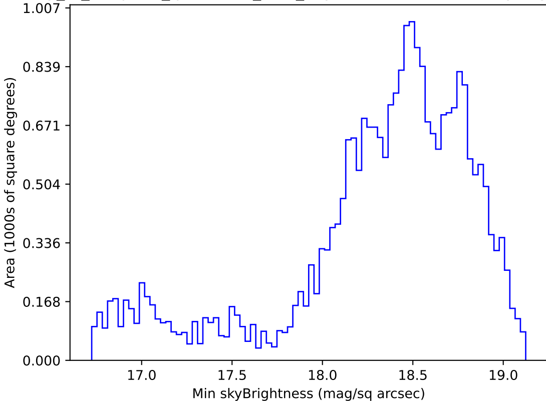
early_ss_template_fpextra2.0_v3.4_10yrs Yr 1 z band: Min skyBrightness
