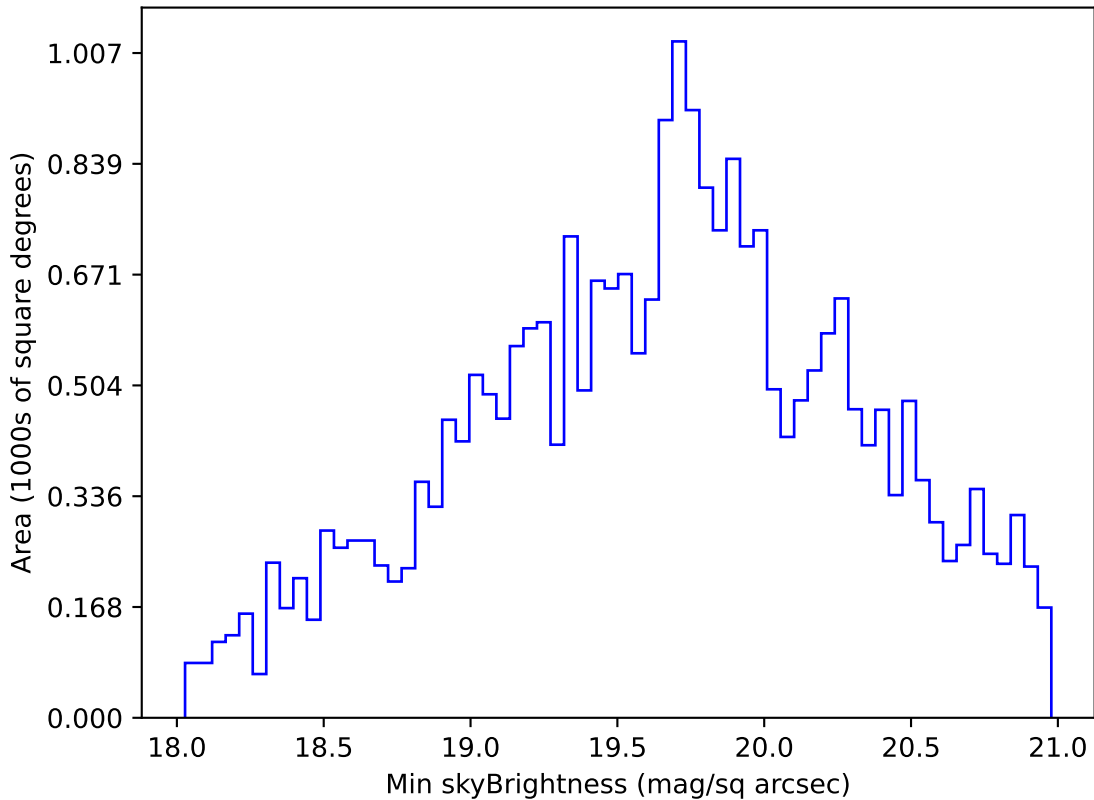
early_ss_template_fpextra2.0_v3.4_10yrs Yr 1 r band: Min skyBrightness
