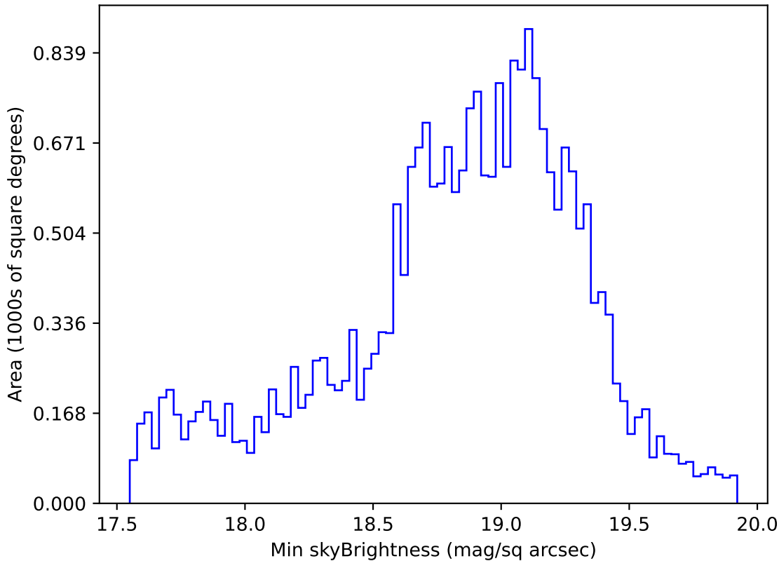
early_ss_template_fpextra2.0_v3.4_10yrs Yr 1 i band: Min skyBrightness
