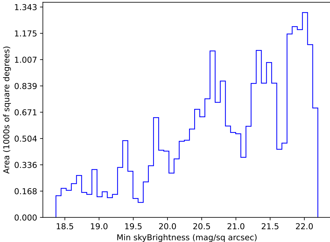
early_ss_template_fpextra2.0_v3.4_10yrs Yr 1 g band: Min skyBrightness
