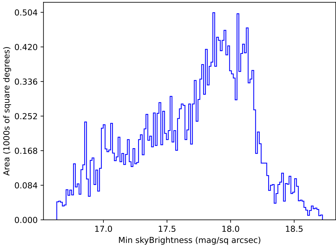
early_ss_template_fpextra2.0_v3.4_10yrs Yr 1 all bands: Min skyBrightness
