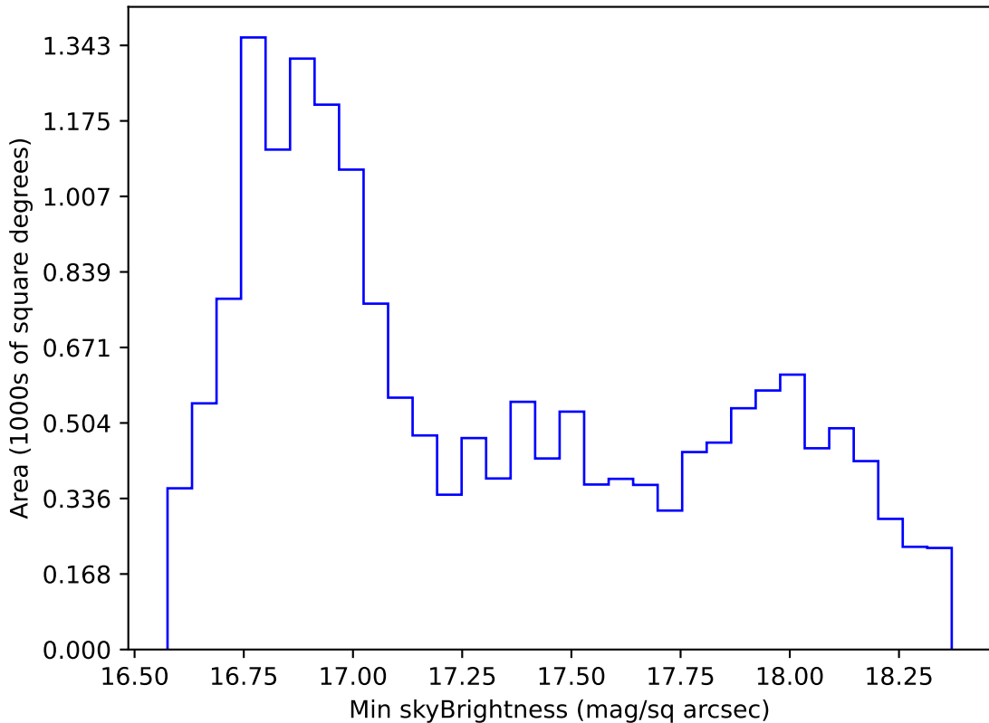
early_ss_template_fpextra2.0_v3.4_10yrs WFD z band: Min skyBrightness
