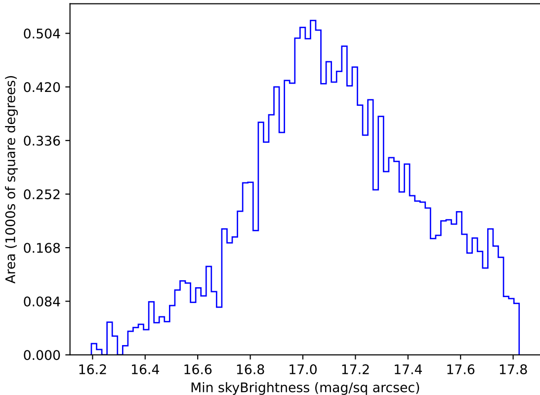
early_ss_template_fpextra2.0_v3.4_10yrs WFD y band: Min skyBrightness
