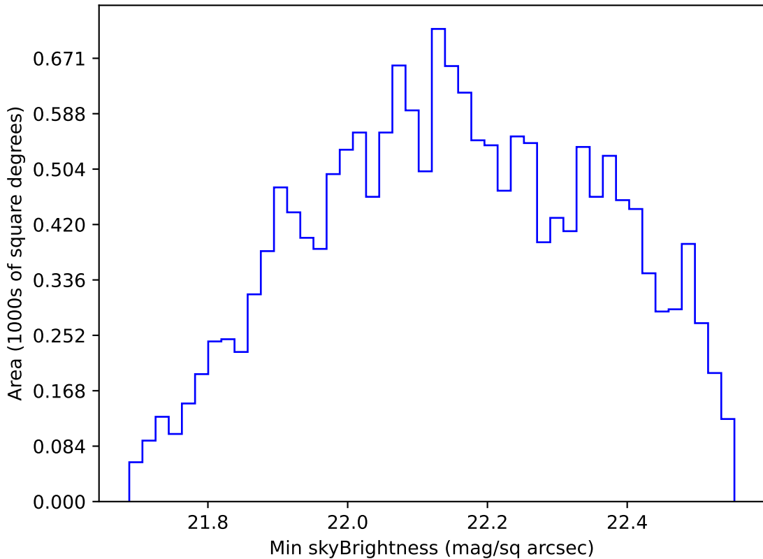
early_ss_template_fpextra2.0_v3.4_10yrs WFD u band: Min skyBrightness
