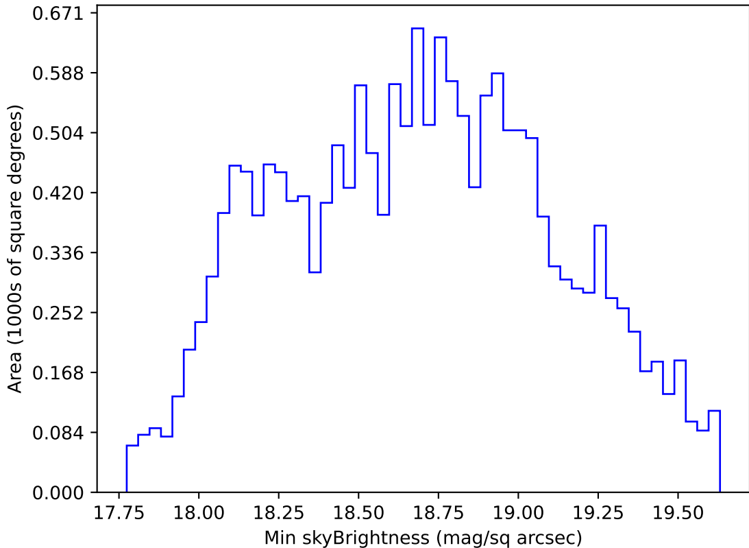
early_ss_template_fpextra2.0_v3.4_10yrs WFD r band: Min skyBrightness
