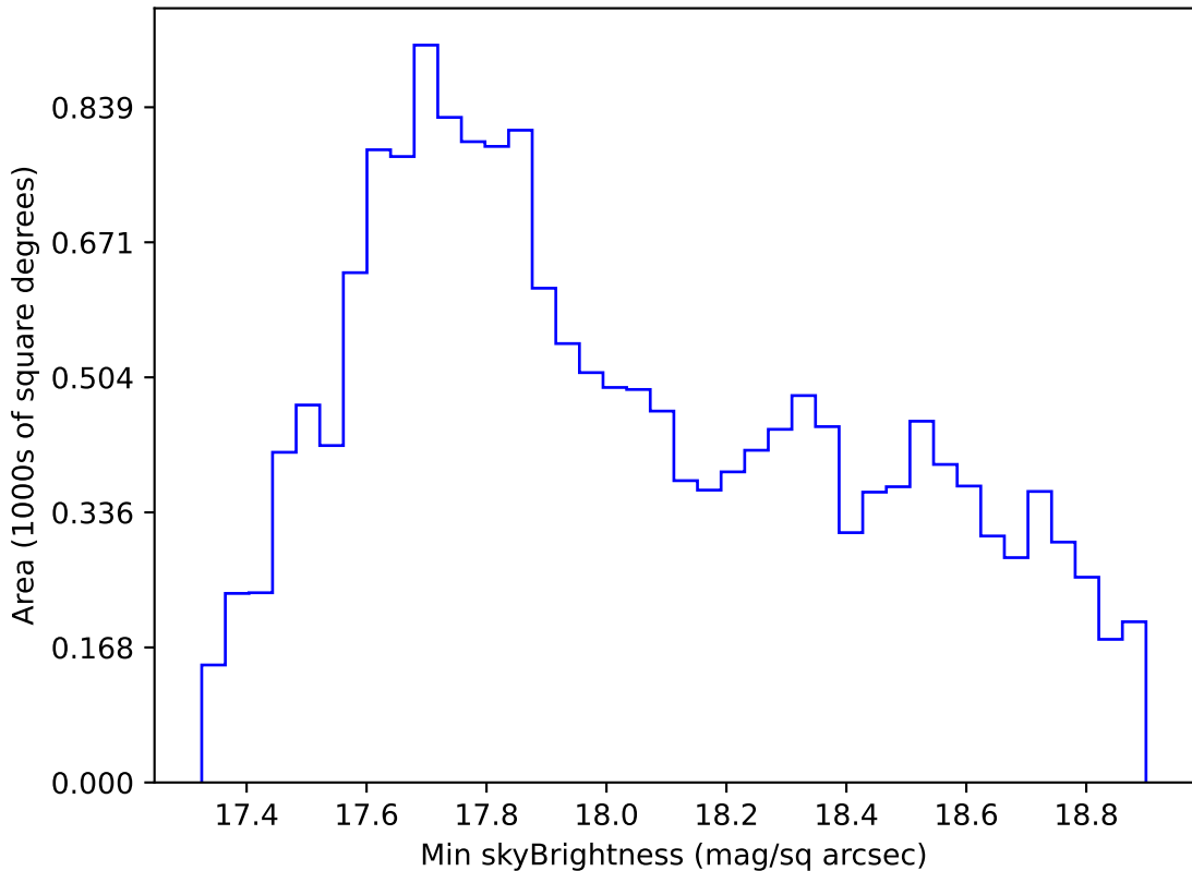
early_ss_template_fpextra2.0_v3.4_10yrs WFD i band: Min skyBrightness
