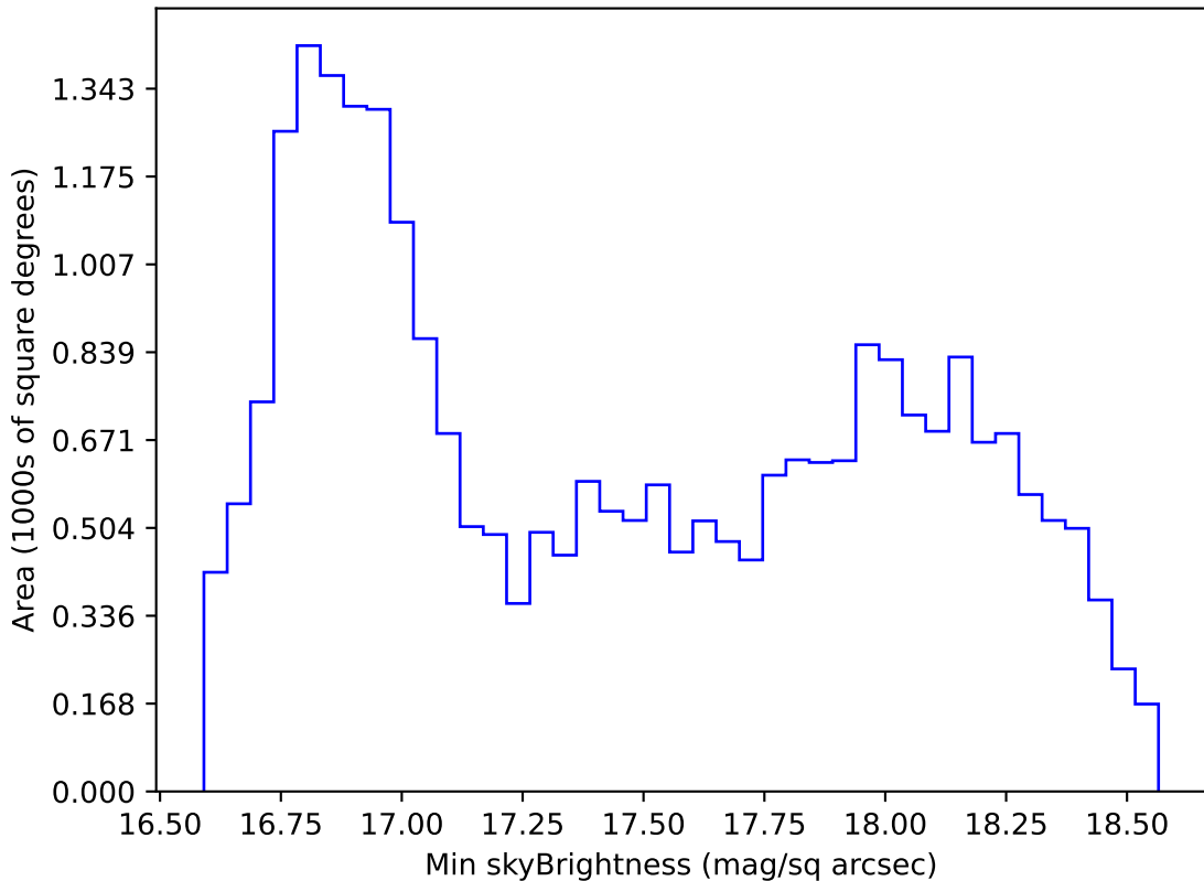
early_ss_template_fpextra2.0_v3.4_10yrs All sky z band: Min skyBrightness
