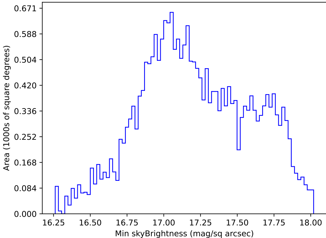
early_ss_template_fpextra2.0_v3.4_10yrs All sky y band: Min skyBrightness
