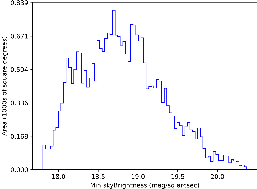
early_ss_template_fpextra2.0_v3.4_10yrs All sky r band: Min skyBrightness
