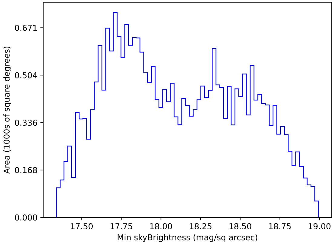
early_ss_template_fpextra2.0_v3.4_10yrs All sky i band: Min skyBrightness
