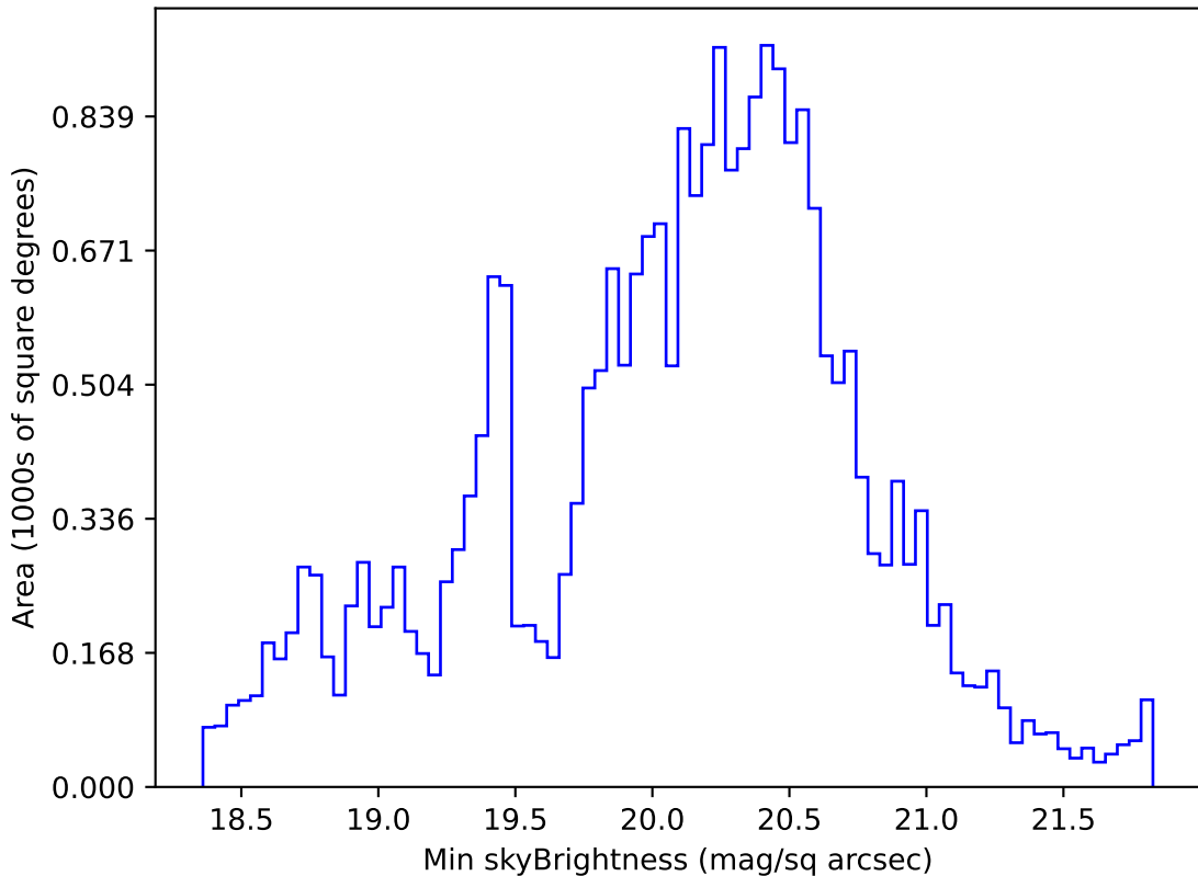
early_ss_template_fpextra2.0_v3.4_10yrs All sky g band: Min skyBrightness
