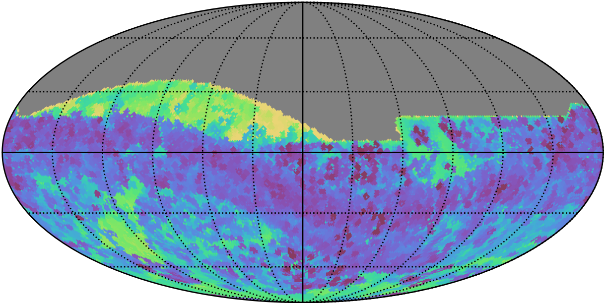
early_ss_template_fpextra2.0_v3.4_10yrs All sky all bands: Min skyBrightness
