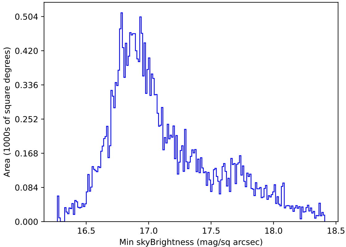
early_ss_template_fpextra2.0_v3.4_10yrs All sky all bands: Min skyBrightness
