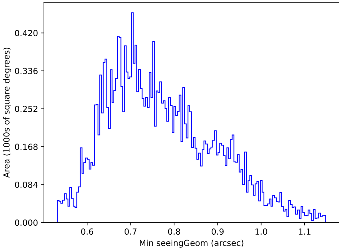
early_ss_template_fpextra2.0_v3.4_10yrs Yr 1 u band: Min seeingGeom
