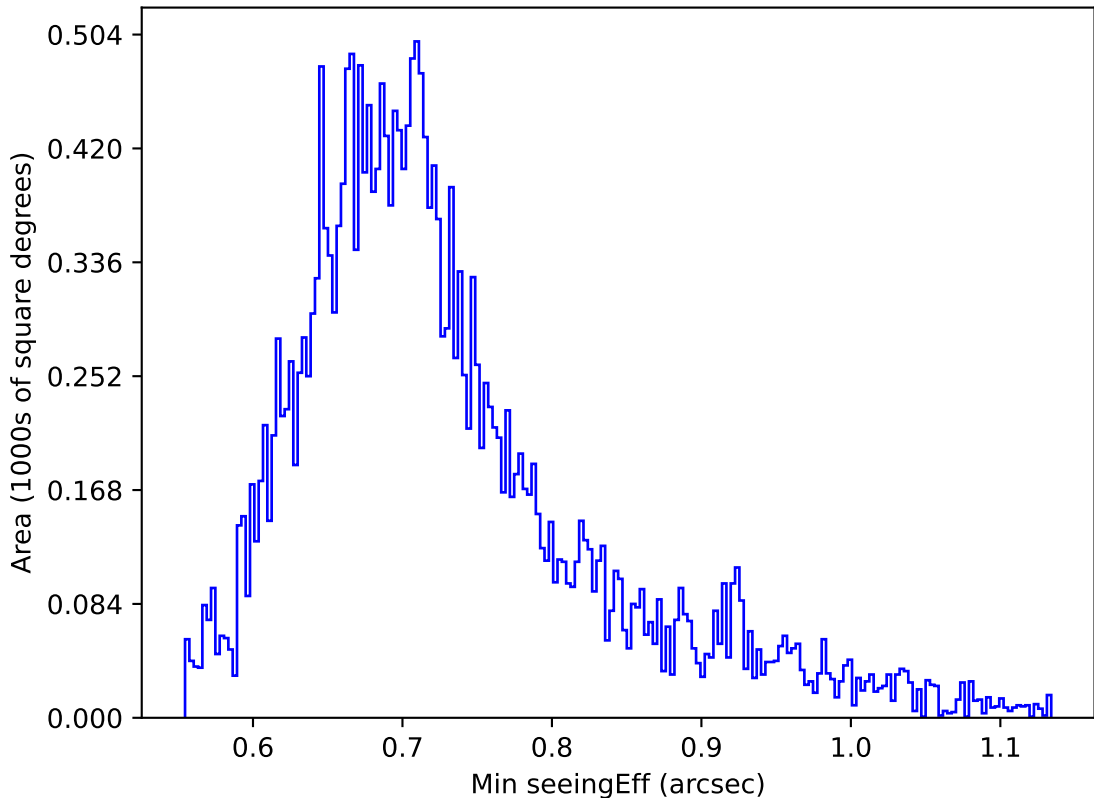
early_ss_template_fpextra2.0_v3.4_10yrs Yr 1 z band: Min seeingEff
