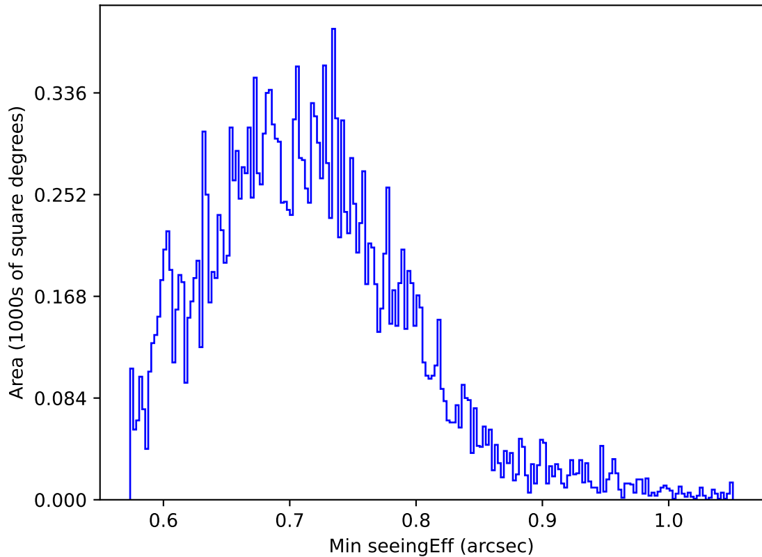
early_ss_template_fpextra2.0_v3.4_10yrs Yr 1 y band: Min seeingEff
