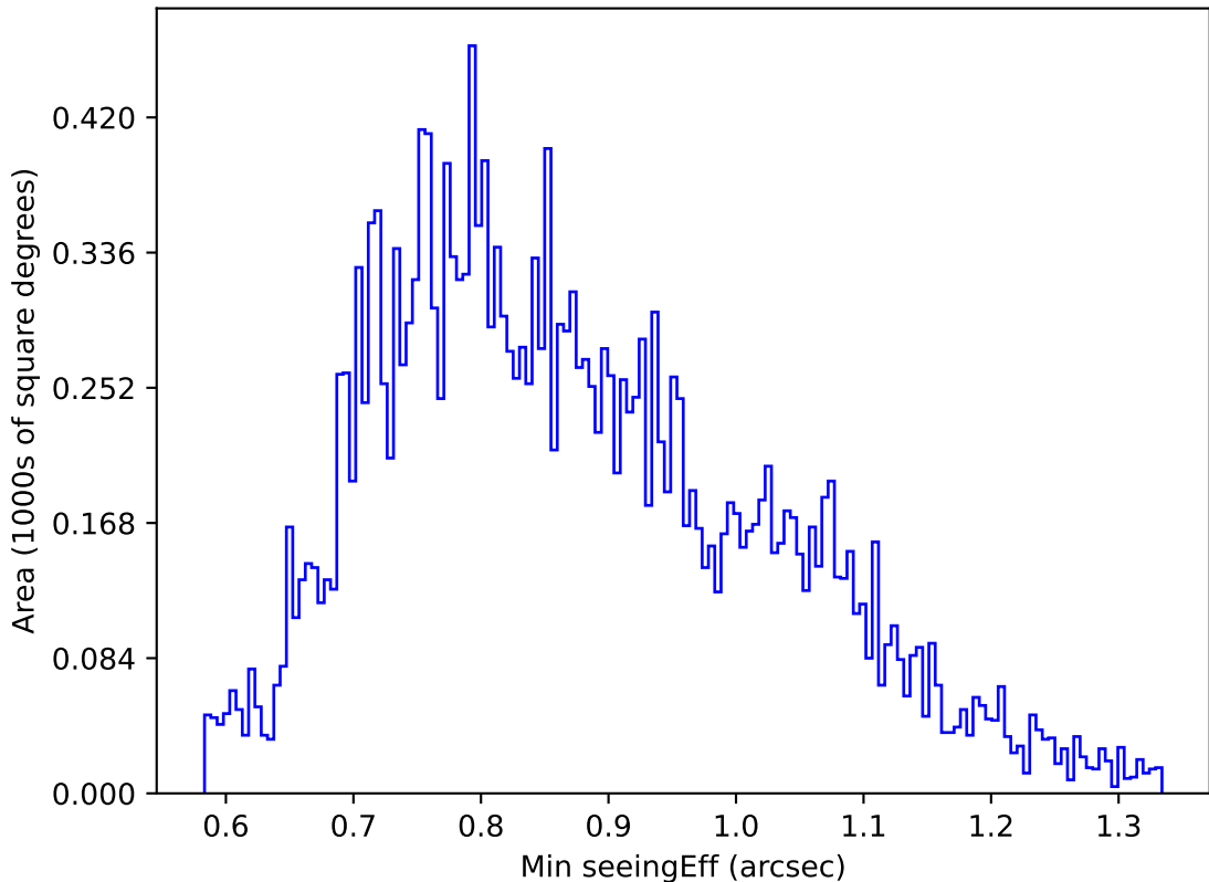
early_ss_template_fpextra2.0_v3.4_10yrs Yr 1 u band: Min seeingEff
