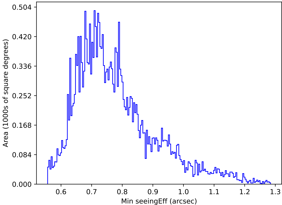
early_ss_template_fpextra2.0_v3.4_10yrs Yr 1 g band: Min seeingEff
