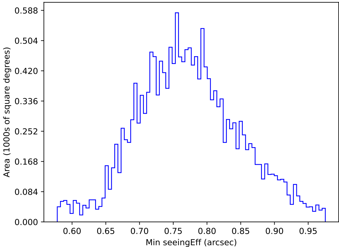
early_ss_template_fpextra2.0_v3.4_10yrs WFD u band: Min seeingEff
