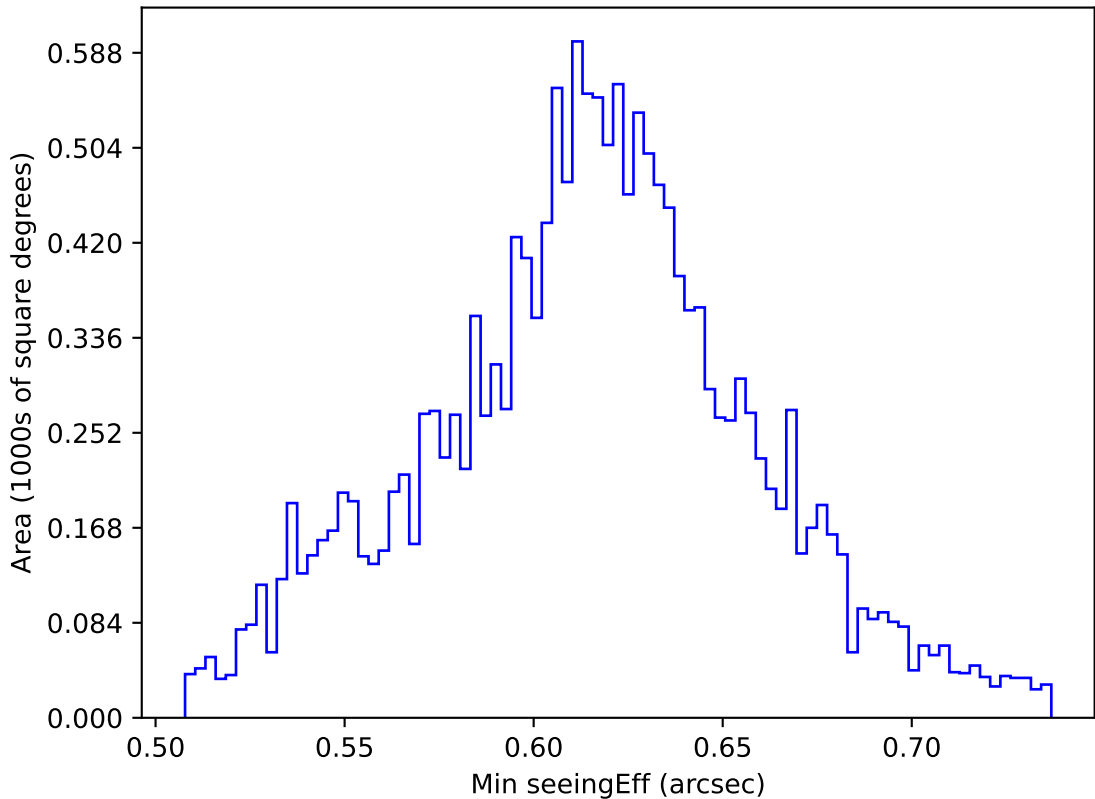
early_ss_template_fpextra2.0_v3.4_10yrs WFD r band: Min seeingEff
