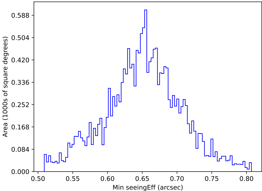
early_ss_template_fpextra2.0_v3.4_10yrs WFD g band: Min seeingEff
