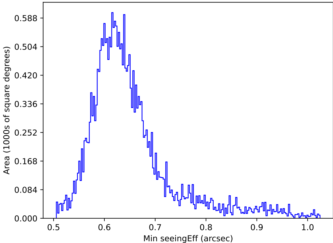
early_ss_template_fpextra2.0_v3.4_10yrs All sky z band: Min seeingEff
