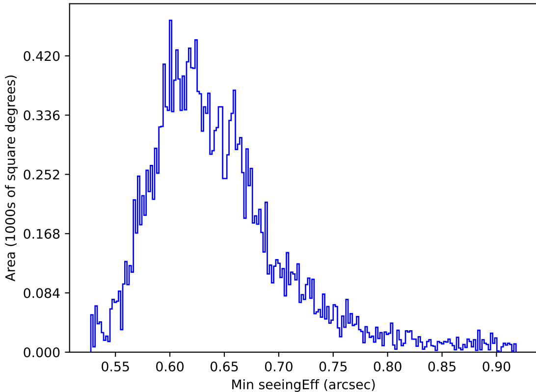
early_ss_template_fpextra2.0_v3.4_10yrs All sky y band: Min seeingEff
