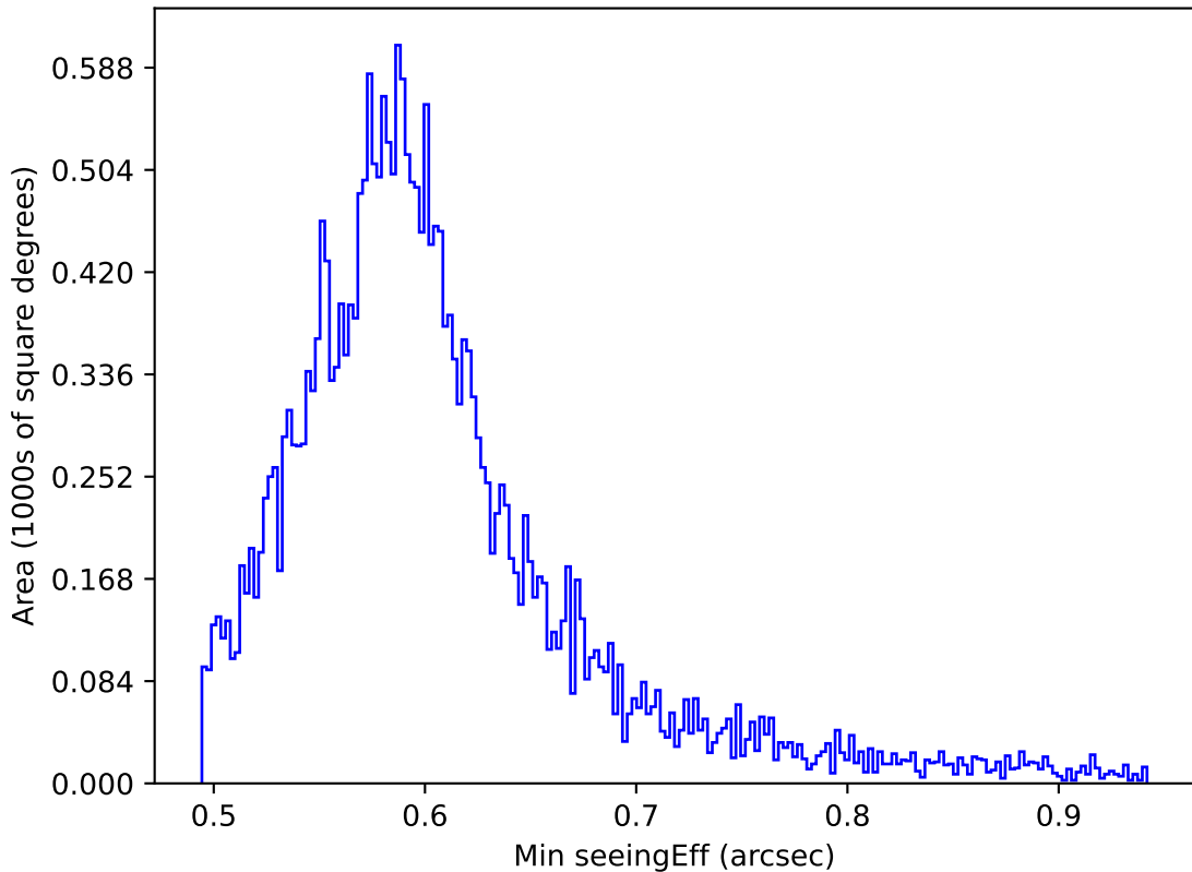
early_ss_template_fpextra2.0_v3.4_10yrs All sky all bands: Min seeingEff
