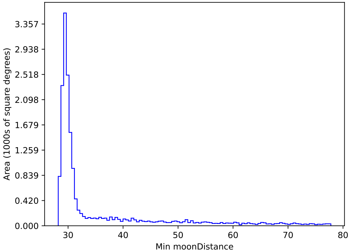
early_ss_template_fpextra2.0_v3.4_10yrs WFD z band: Min moonDistance
